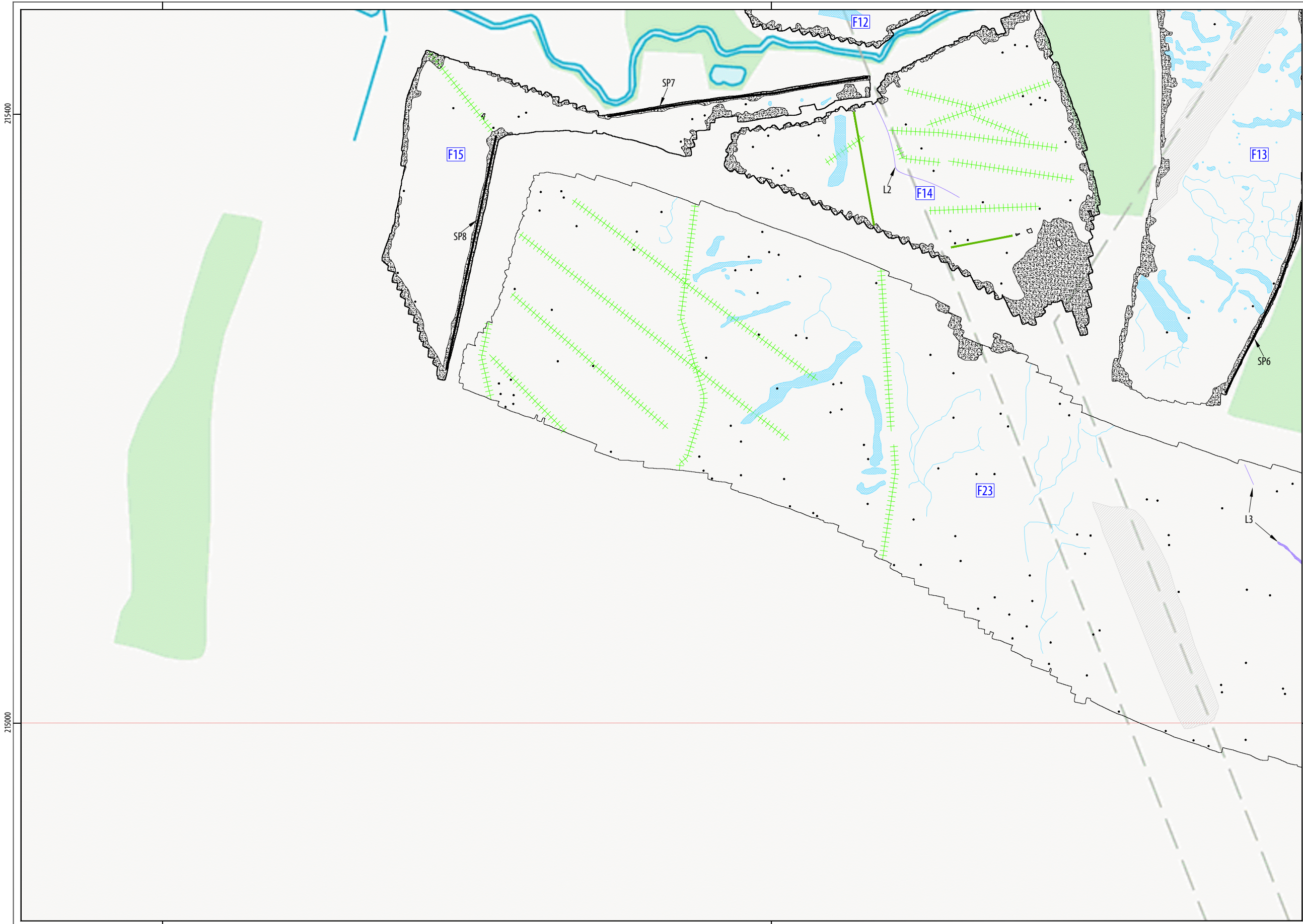
ILLUS 24 Interpretation of magnetometer data; Area 4
