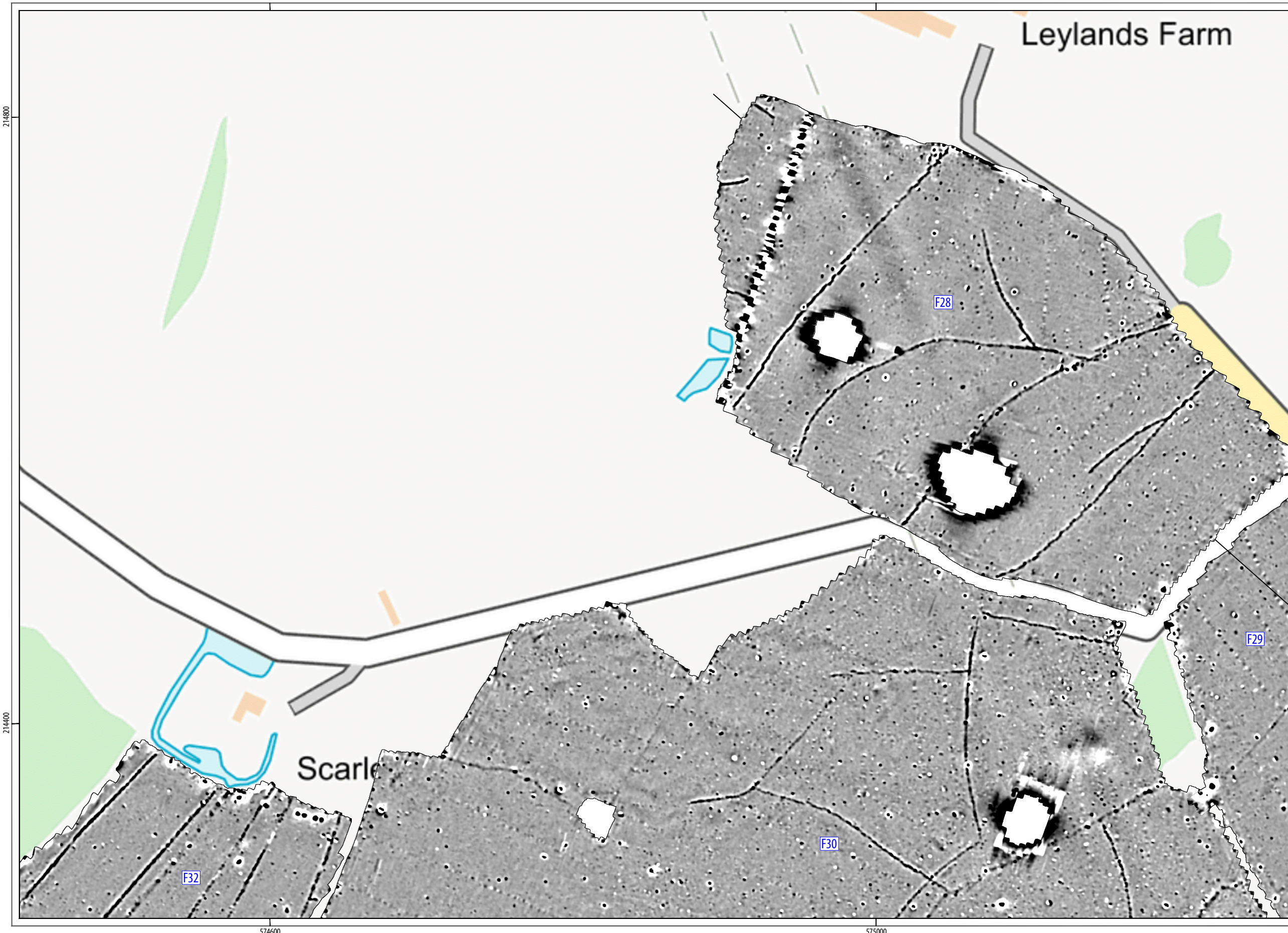
ILLUS 31 Processed greyscale magnetometer data; Area 7
