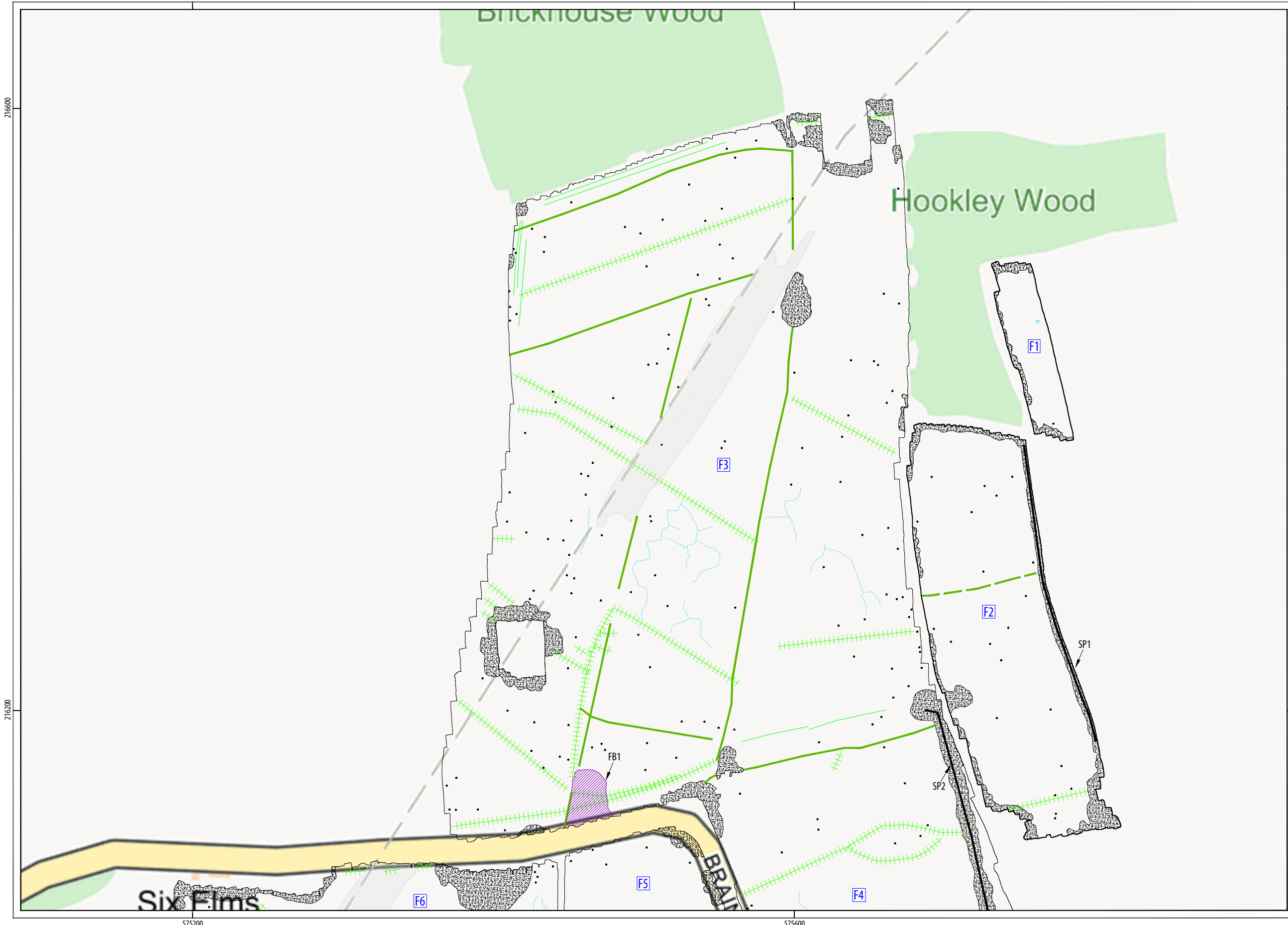
ILLUS 15 Interpretation of magnetometer data; Area 1
