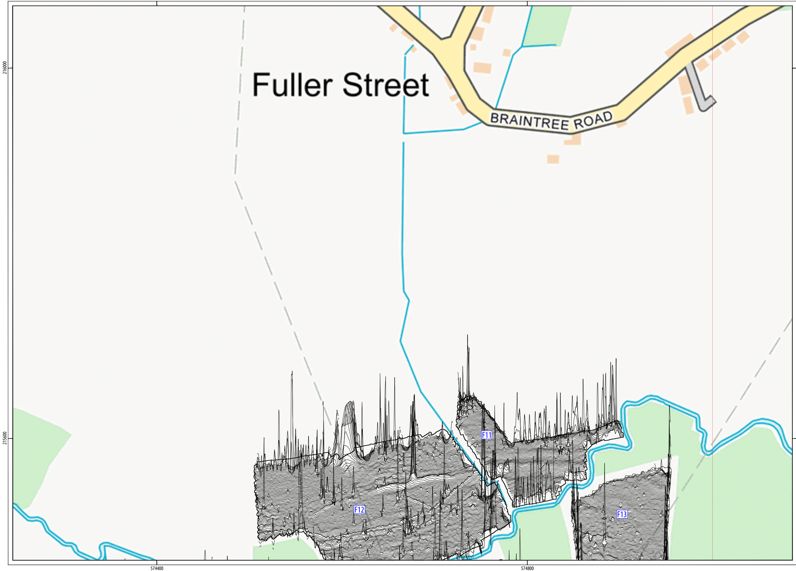
ILLUS 17 XY trace plot of minimally processed magnetometer data; Area 2
