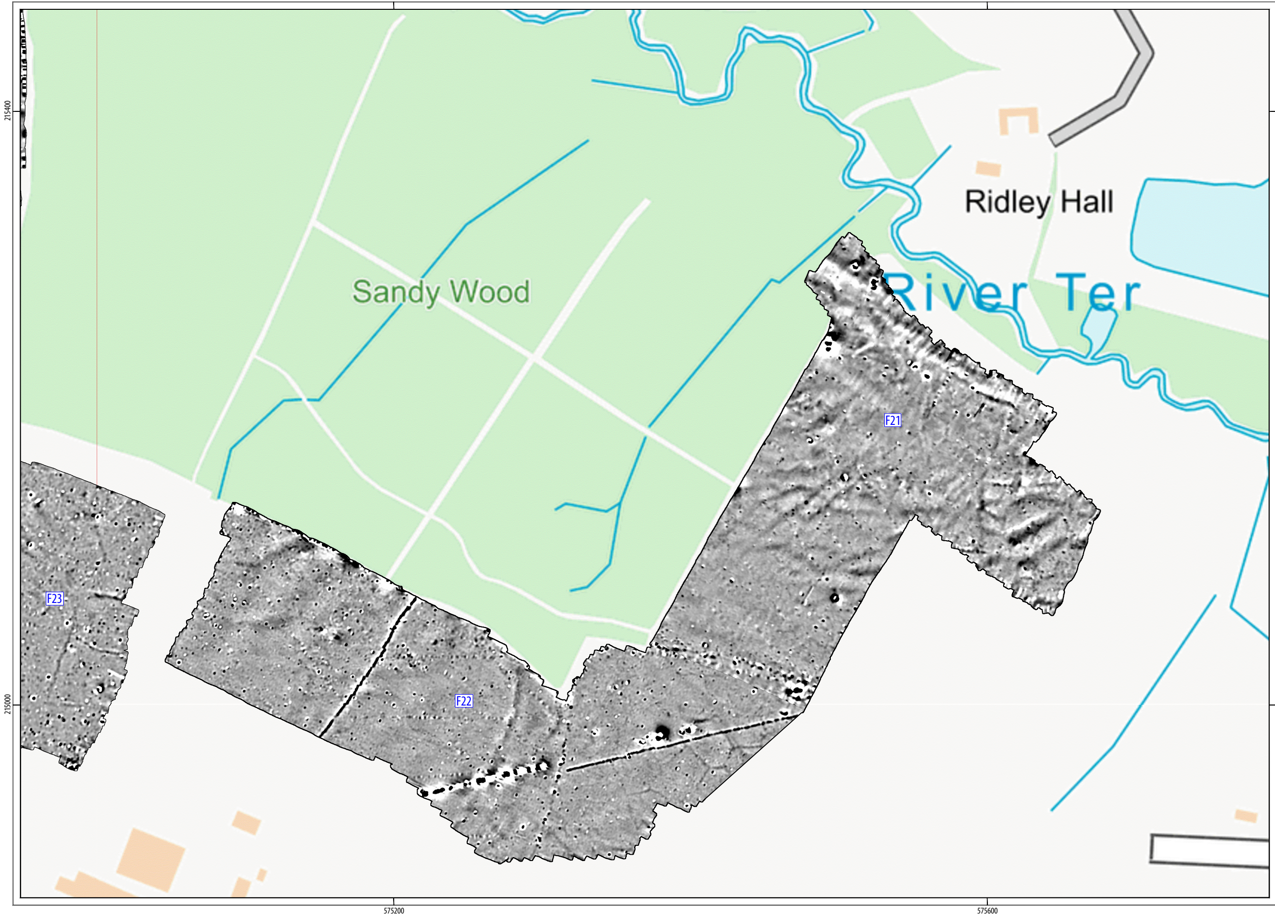
ILLUS 25 Processed greyscale magnetometer data; Area 5
