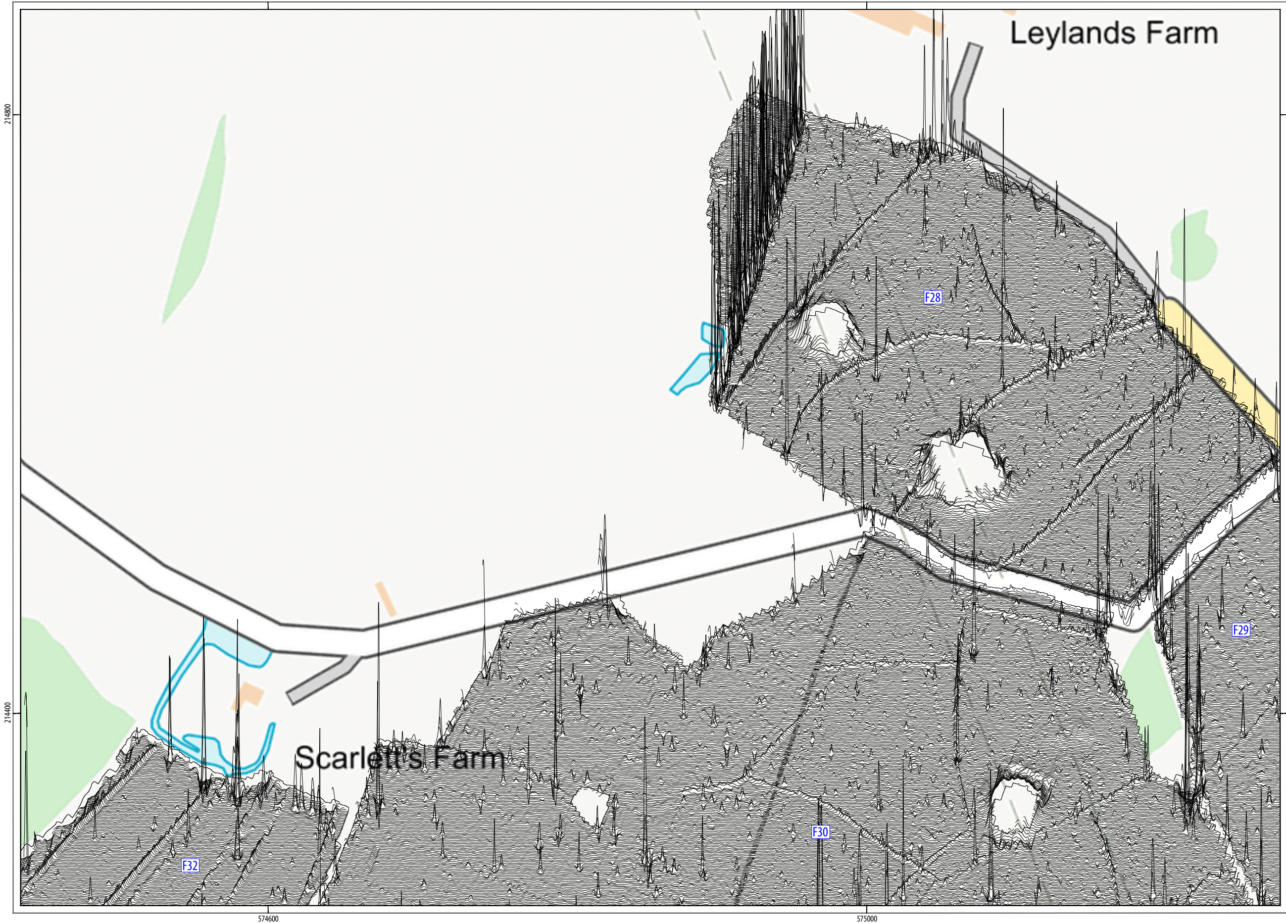
ILLUS 32 XY trace plot of minimally processed magnetometer data; Area 7
