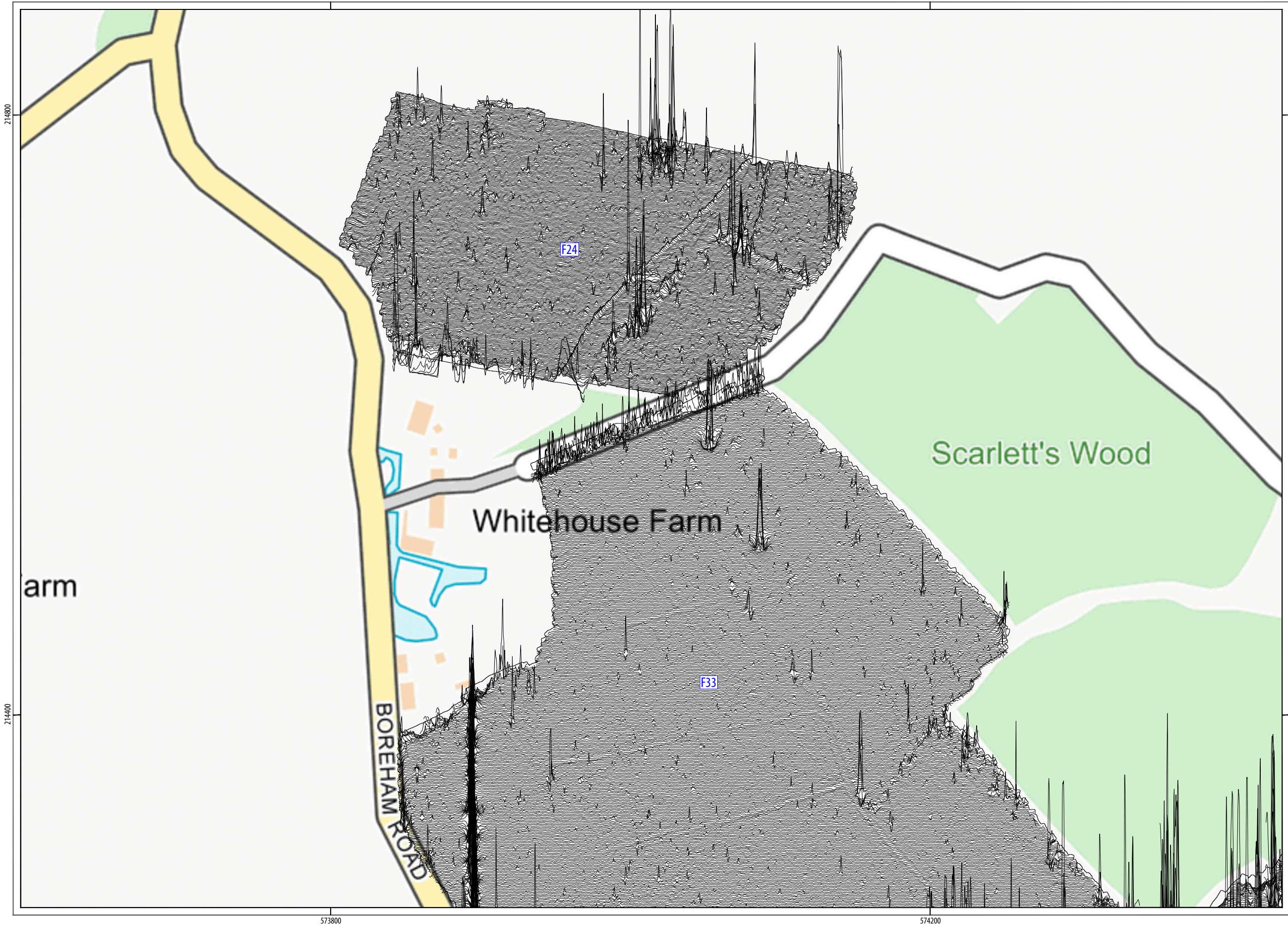
ILLUS 29 XY trace plot of minimally processed magnetometer data; Area 6
