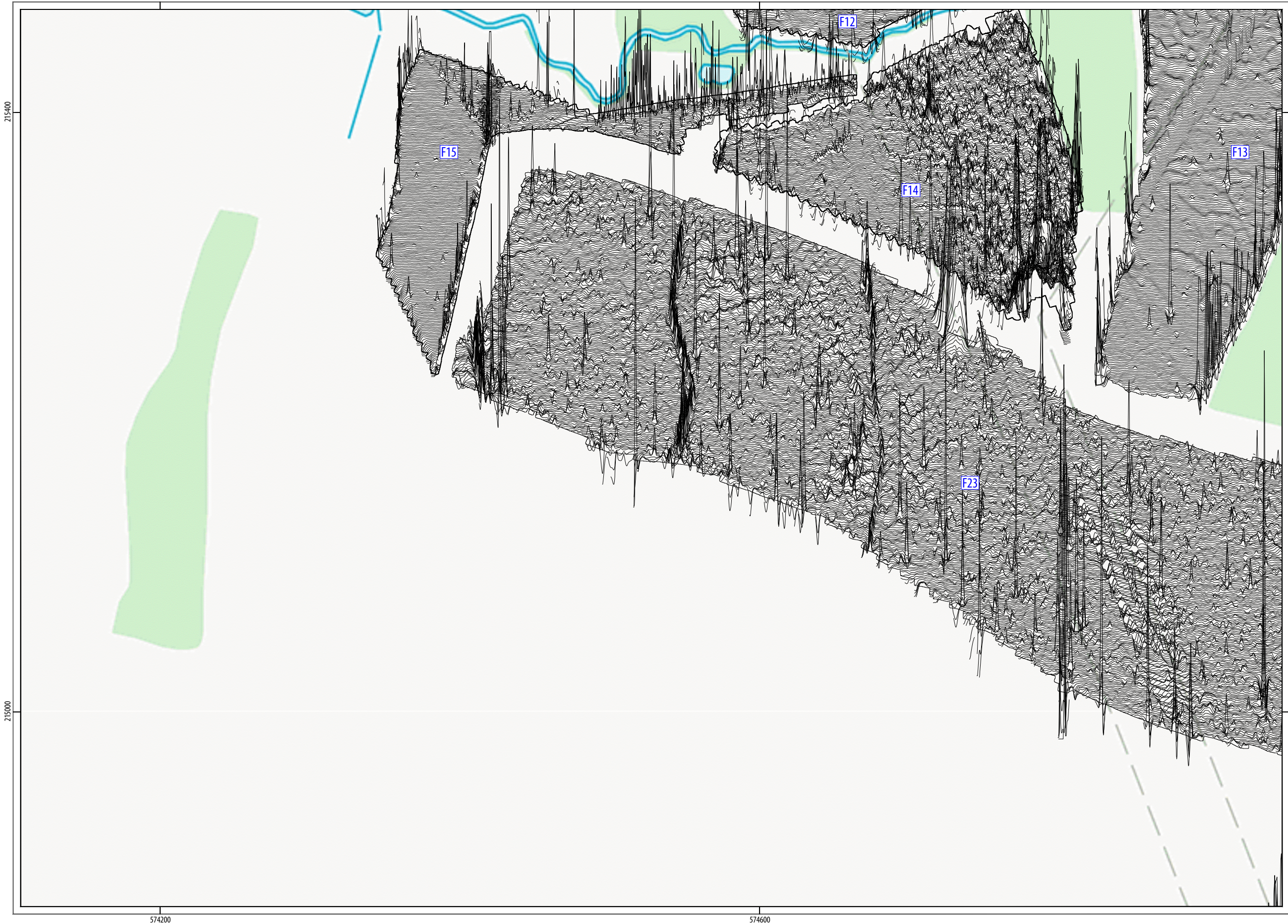
ILLUS 23 XY trace plot of minimally processed magnetometer data; Area 4
